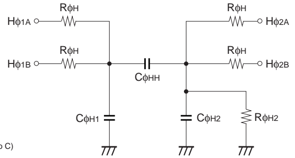
Horizontal transfer clock equivalent circuit
