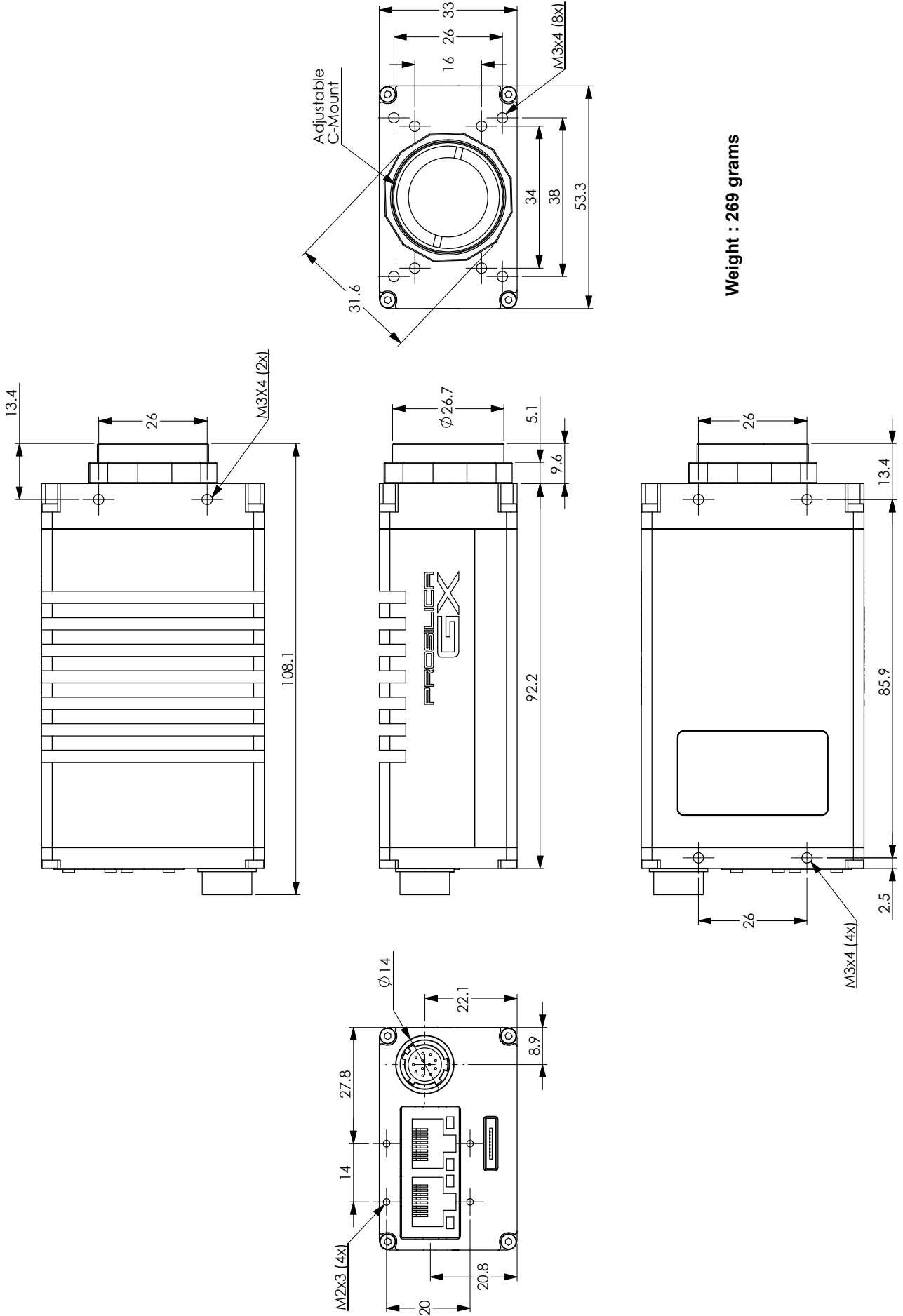
Prosilica GX1920 / GX1920C
