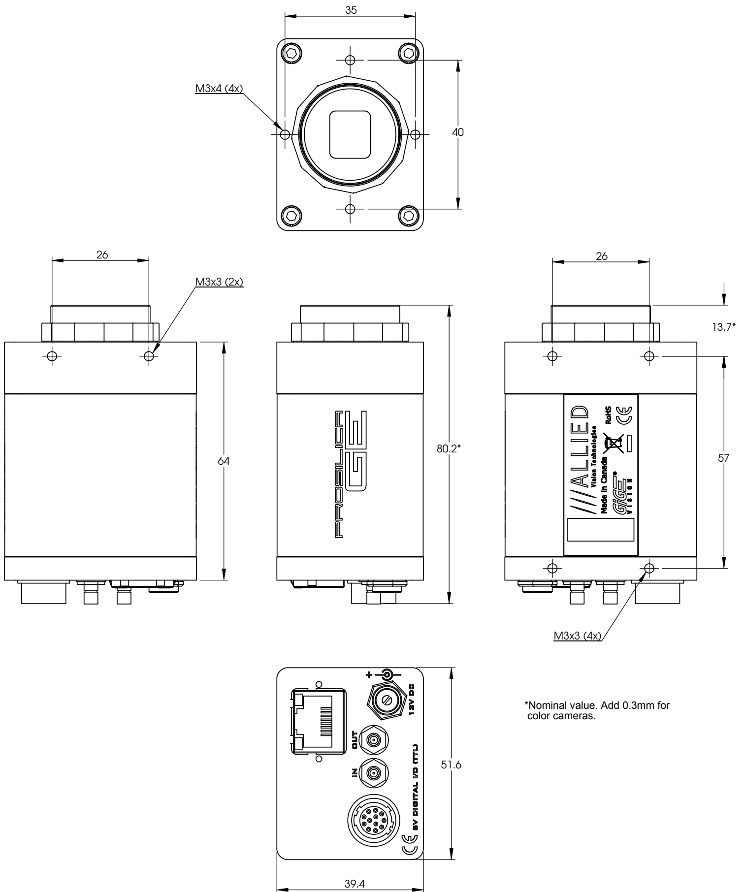
Prosilica GE1660
